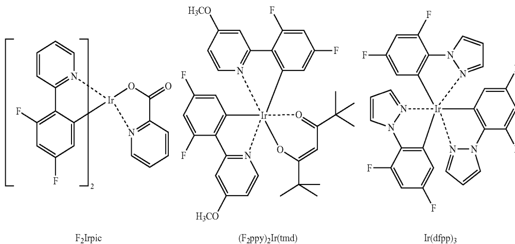
F 2 Irpic
