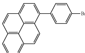
Synthesis Example 29
