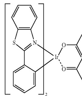
Ir(BT) 2 (acac)
