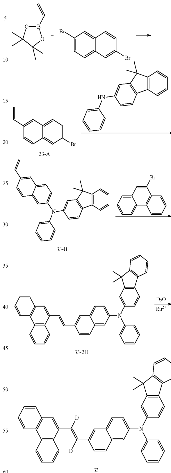
Reaction scheme 2
