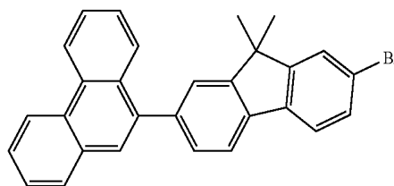
Synthesis Example 28
