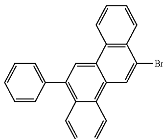
Synthesis Example 25
